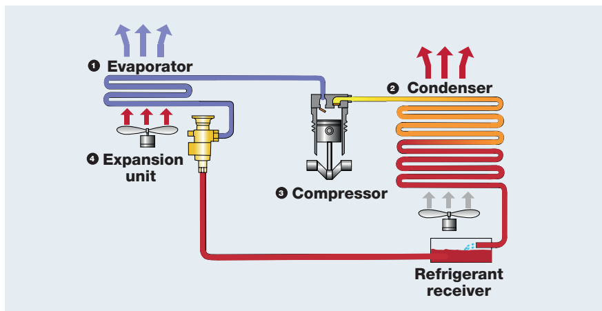
Simple, schematic refrigerant circuit
