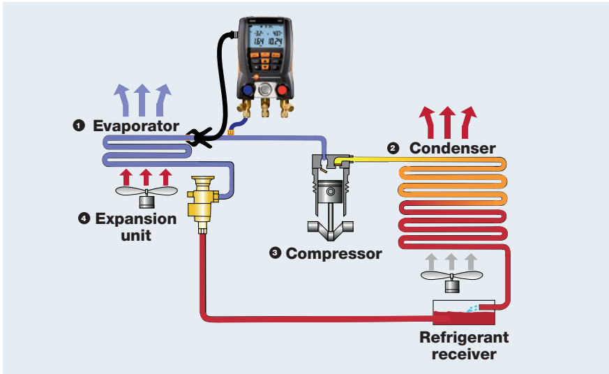
Determination of evaporator superheating
