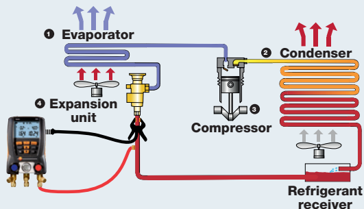
Determination of subcooling before the expansion valve
